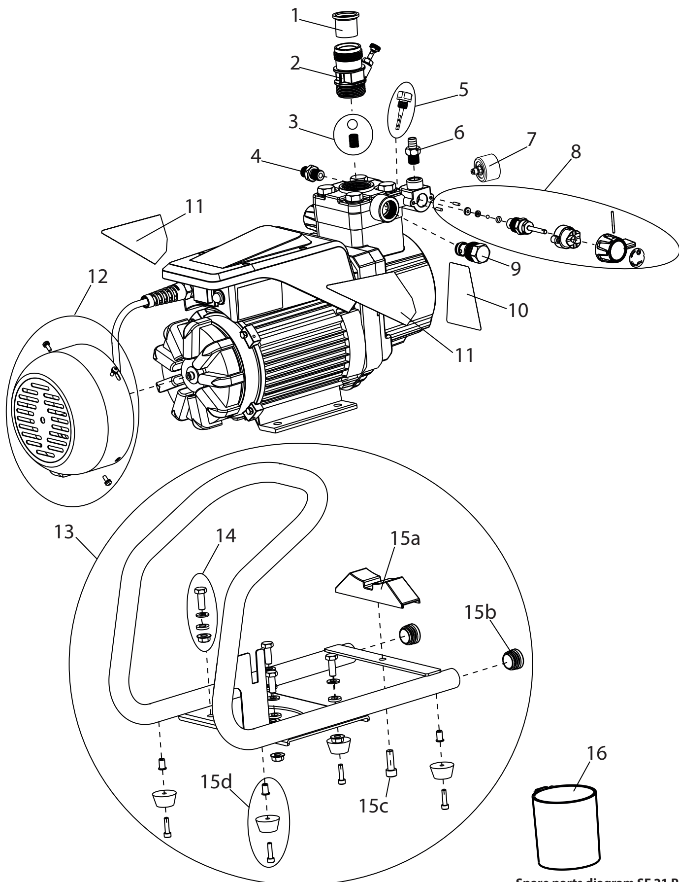
Spare parts diagram SF 21 Pro
